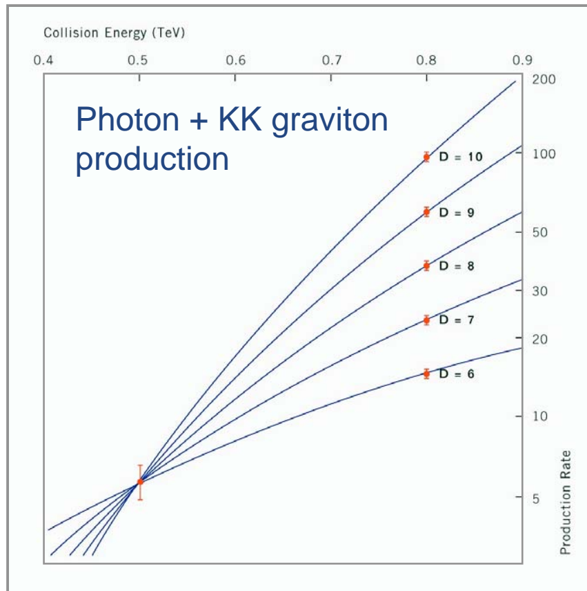
Dimension Counting at ILC
