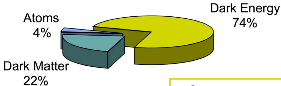
Composition of Universe
