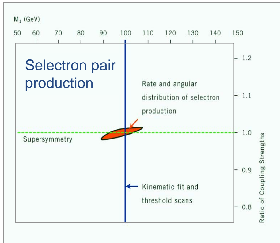
SUSY Couplings at ILC
